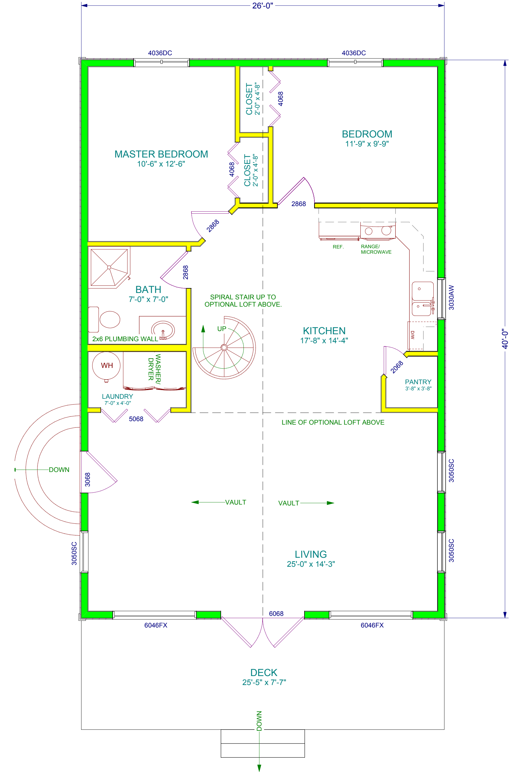
MAIN FLOOR PLAN SCALE: 1/4" = 1'-0"
